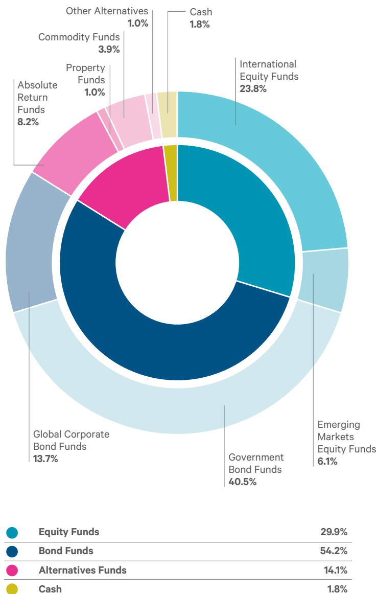
Figure 2: Asset Allocation
